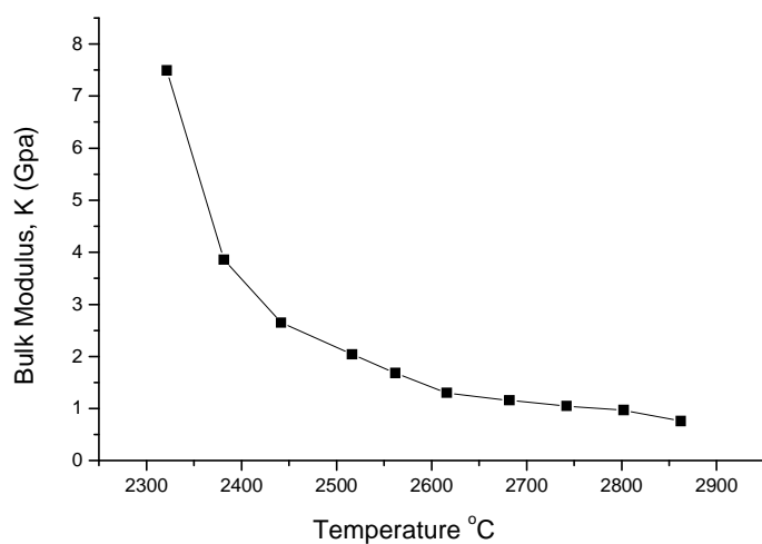
Figure 12: Bulk modulus against temperature (sample 10)
