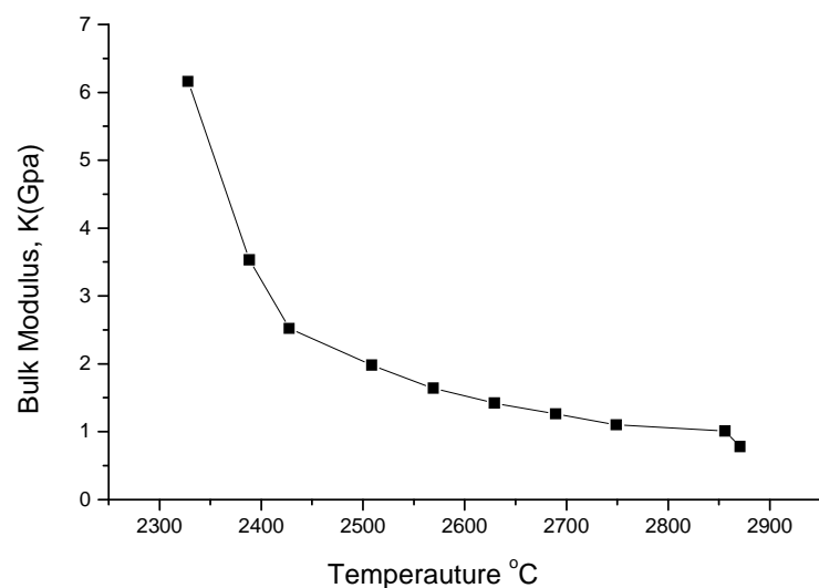
Figure 13: Bulk modulus against temperature (sample 11)
