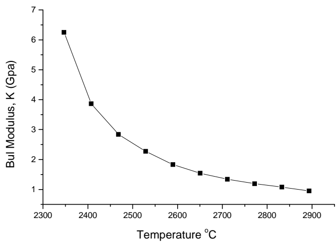
Figure 27: Bulk modulus against temperature (sample 25)
