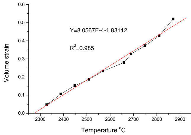
Figure 2: A representation of volume strain plotted against temperature (sample 1) The above graph show that an increase in strain results in a lowering of \alpha K_T at high value of temperature T.
