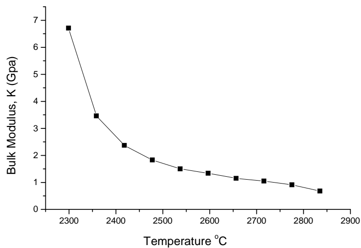
Figure 7: Bulk modulus against temperature (sample 5)
