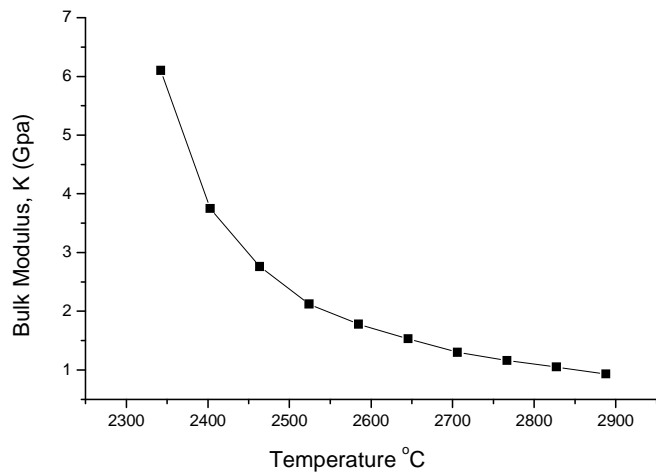
Figure 22: Bulk modulus against temperature (sample 20)
