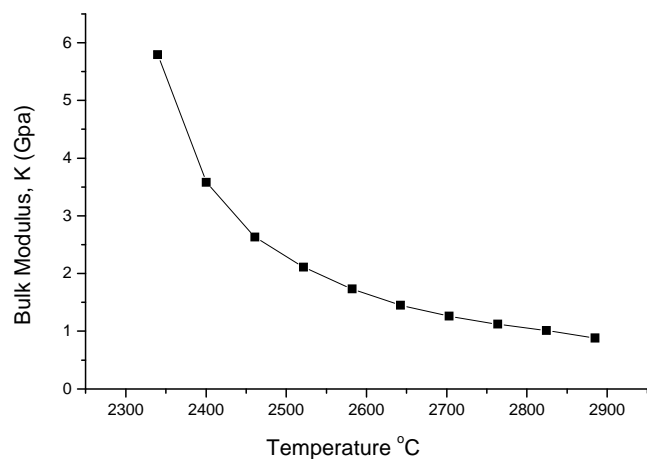
Figure 21: Bulk modulus against temperature (sample 19)
