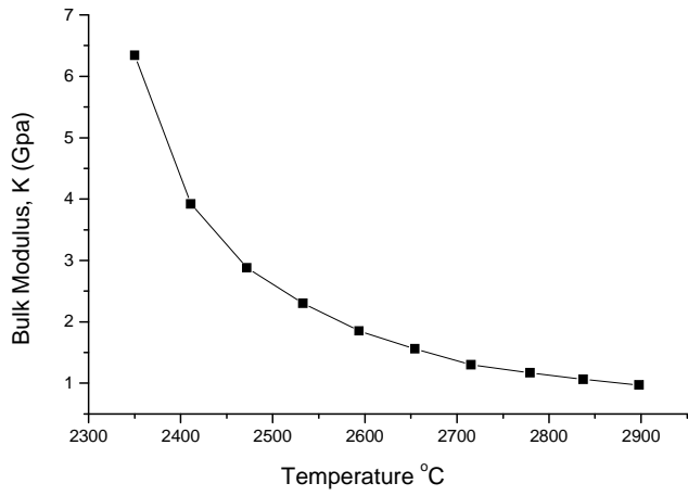
Figure 28: Bulk modulus against temperature (sample 26)
