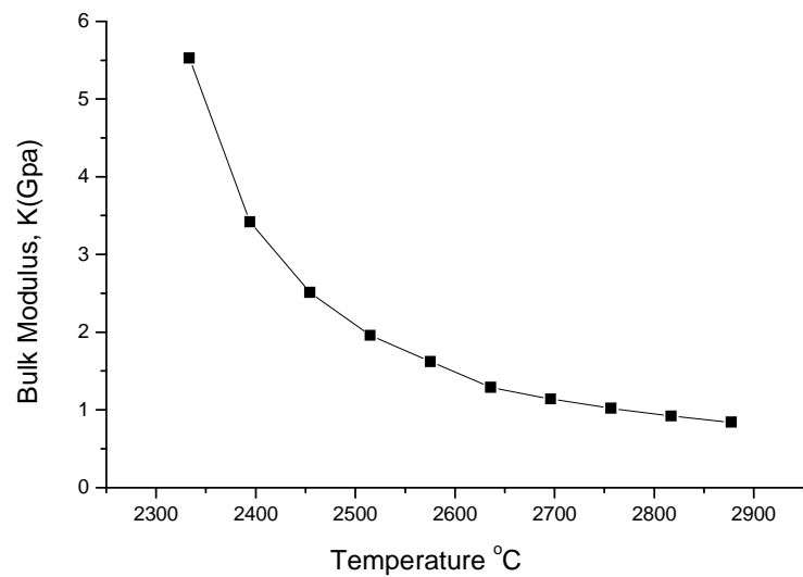
Figure 16: Bulk modulus against temperature (sample 14)
