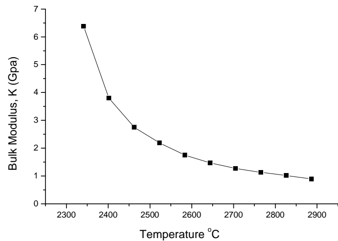
Figure 21: Bulk modulus against temperature (sample 19)
