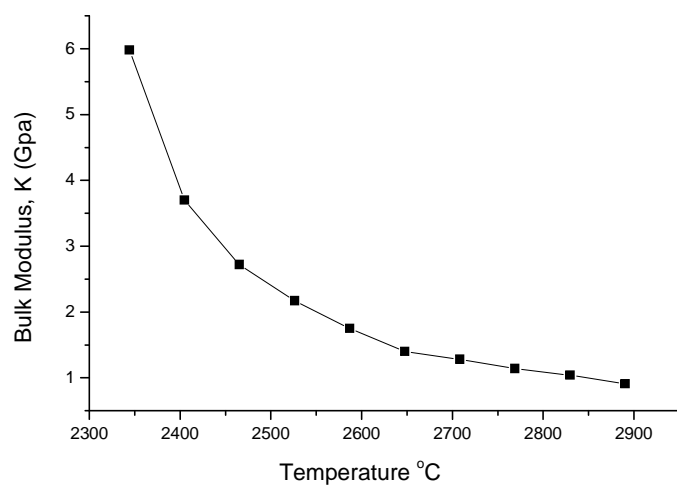
Figure 23: Bulk modulus against temperature (sample 21)
