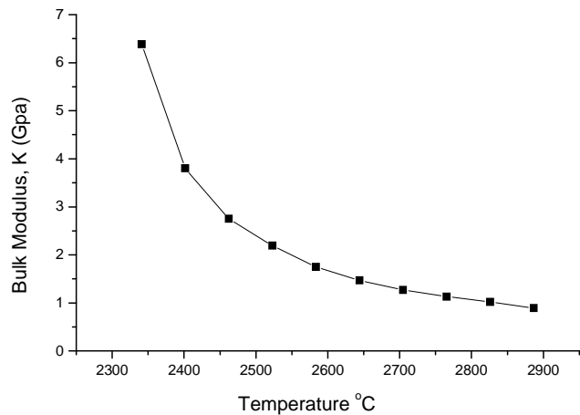
Figure 20: Bulk modulus against temperature (sample 18)
