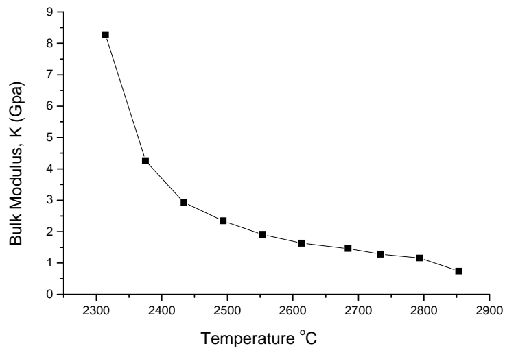
Figure 10: Bulk modulus against temperature (sample 8)
