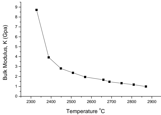
Figure 3: Bulk modulus against temperature (sample 1)
