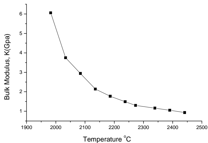
Figure 24: Bulk modulus against temperature (sample 22)
