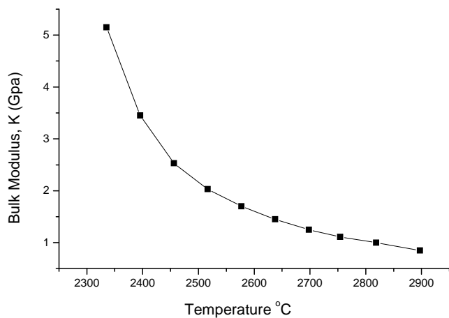
Figure 17: Bulk modulus against temperature (sample 15)
