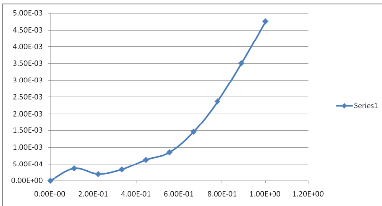
Fig 8: I.V curve for the solar cell in dark
