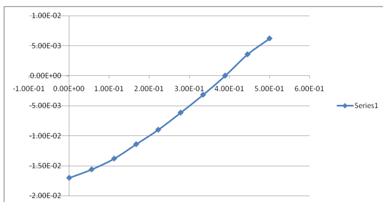
Fig 9: I.V curve for the solar cell in light.
