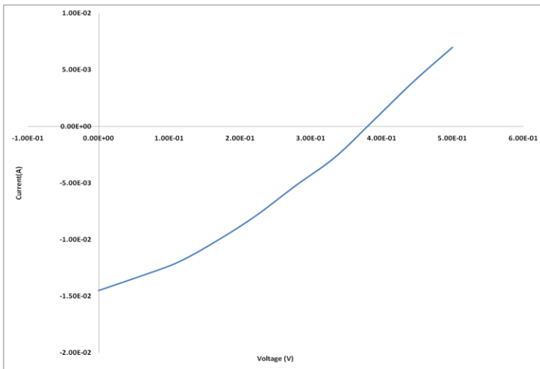
Fig 7: I.V curve for the solar cell in light.
