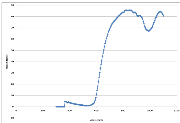
Fig 5 Graph of transmittance of liquid in zobo dye
