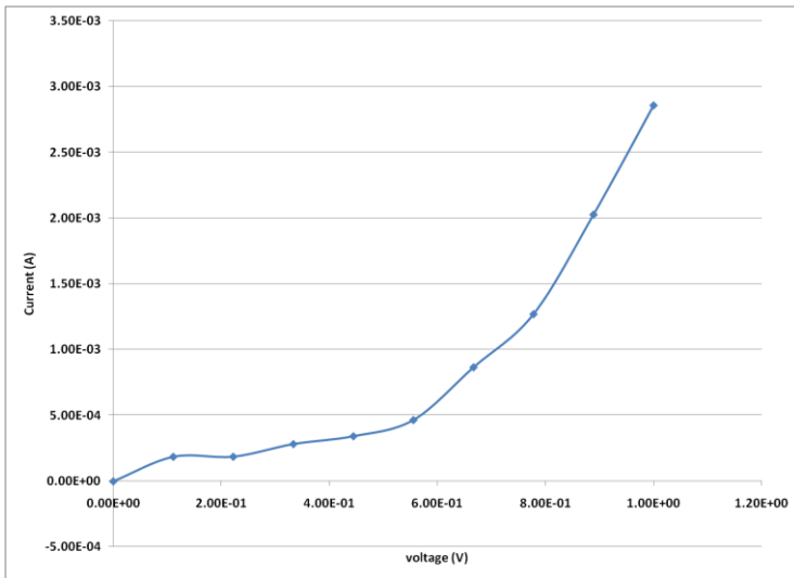
Fig 6: I.V curve for the solar cell in dark
