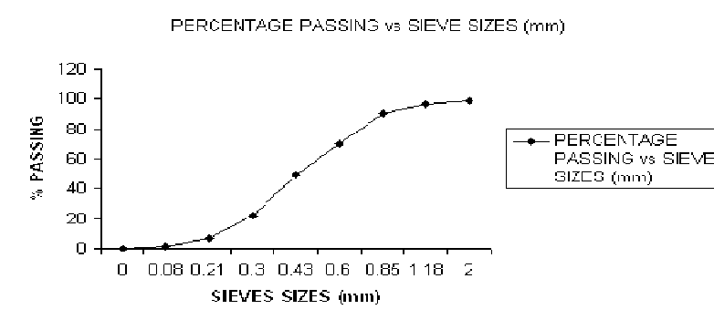
Figure 4: Grading curve for the fine aggregate
