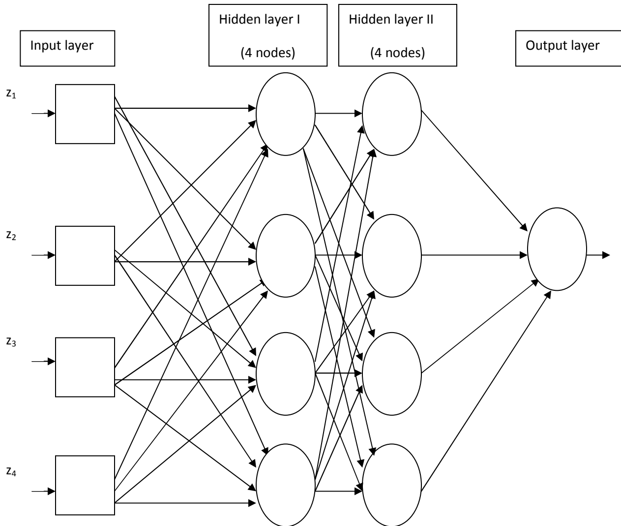
Figure 3: The Four-input, 4 layers feed foreword neural network model
