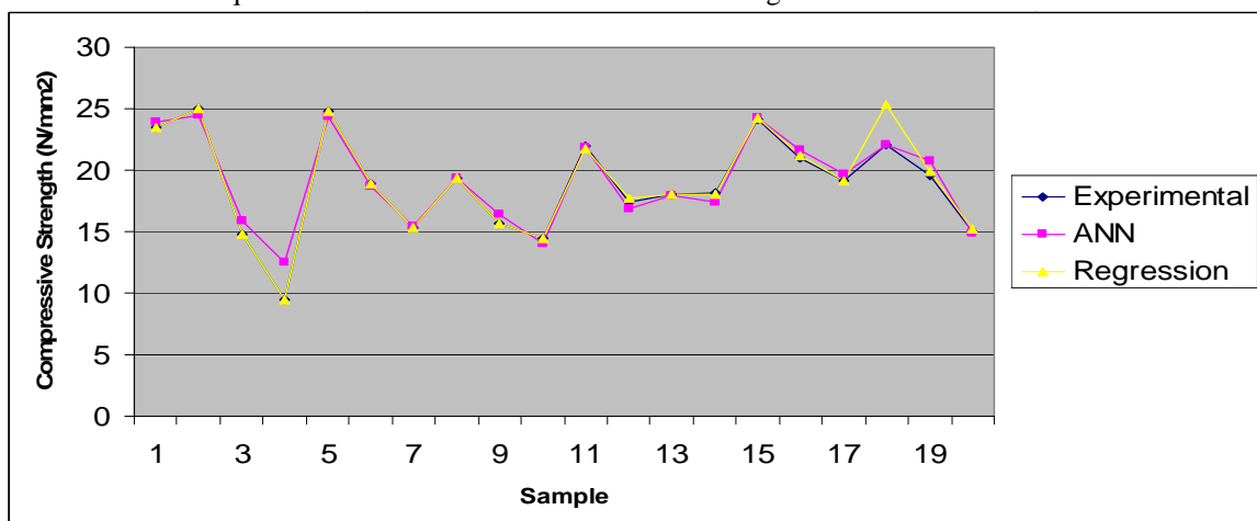
Figure 6: Comparison of ANN with experimental results and regression model prediction (washed gravel)
