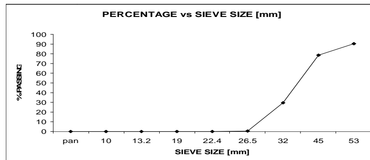
Figure 5: Grading curve for the local gravel
