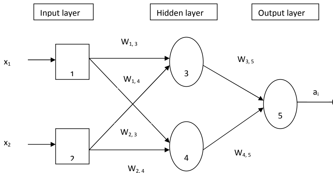
Figure 2: Two-input feed forward neural network model
