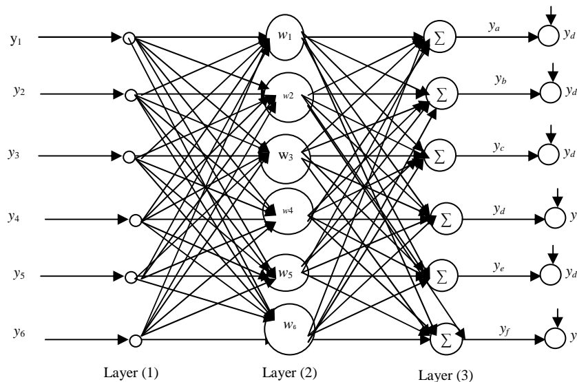
Figure 3.2: The structure of Neuro Fuzzy model.
